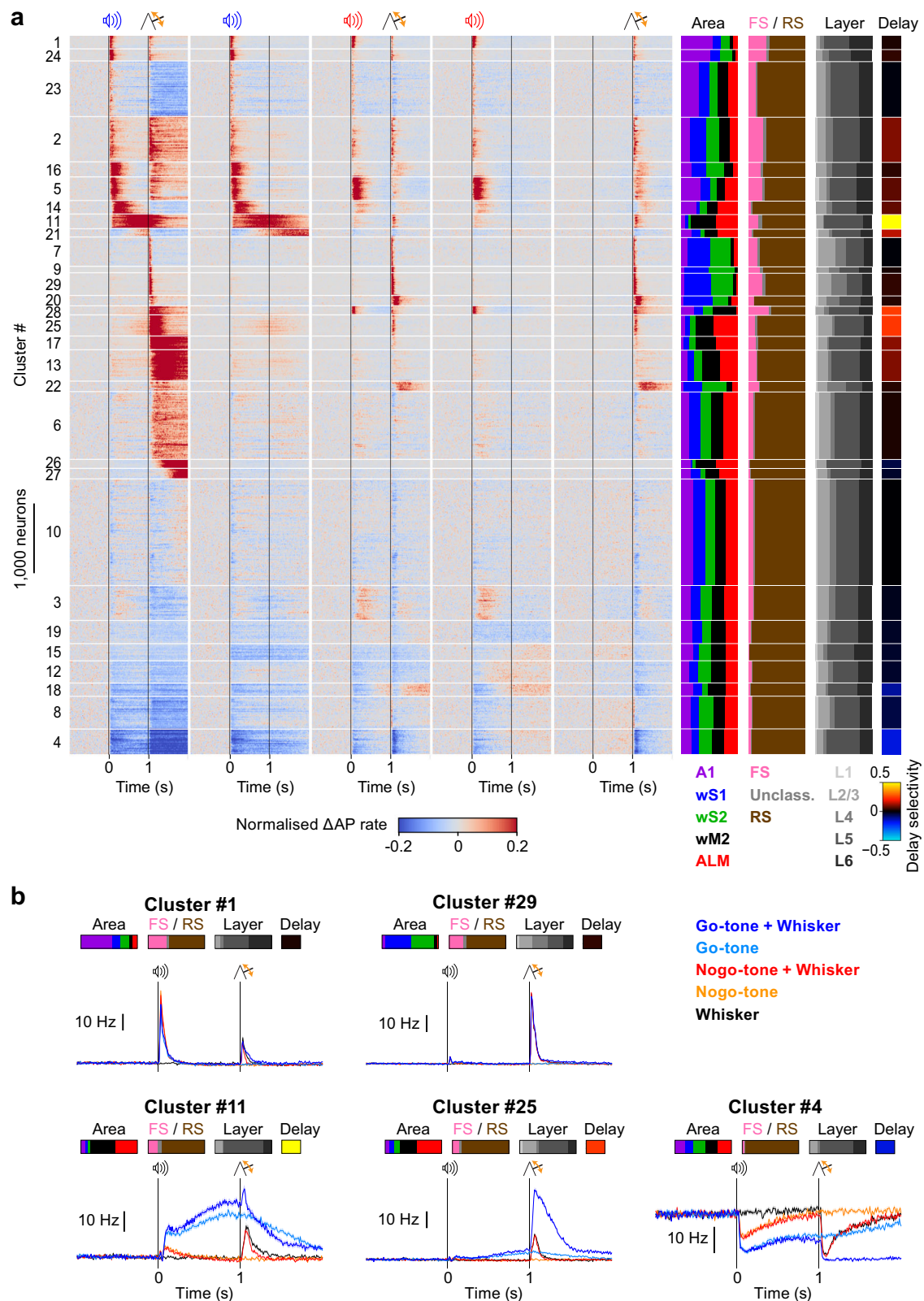
Fig. 4 | Diverse patterns of neuronal activity distributed across cortical regions, layers, and cell classes. a The averaged PSTHs for each recorded neuron in the five types of correctly executed trials were baseline subtracted, normalized, and clustered using a Gaussian mixture model after spectral embedding of the principal components, with the number of clusters determined by the minimum Bayesian Information Criterion. This identified 29 clusters each containing neurons with similar dynamics, but distributed across different cortical areas (A1, wS1, wS2, wM2,
