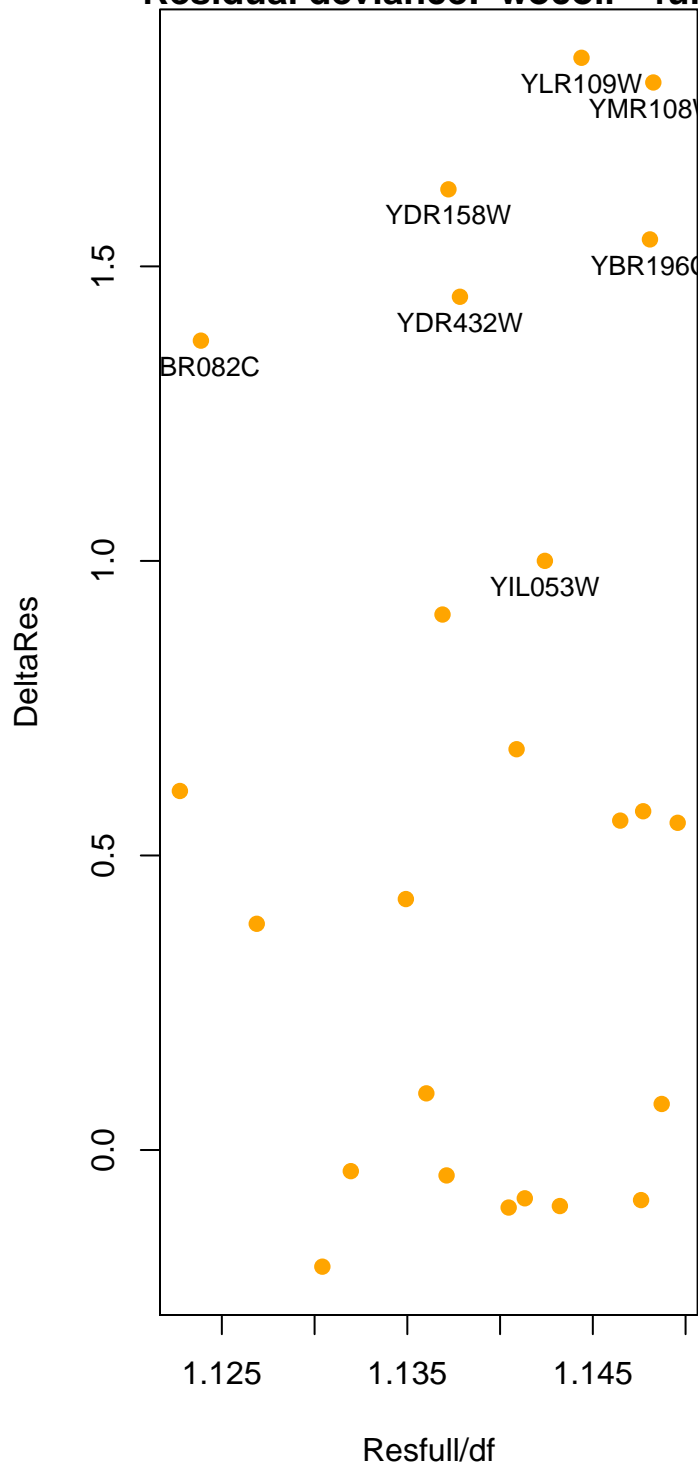
Residual deviance: 'wocoll'-'full'
